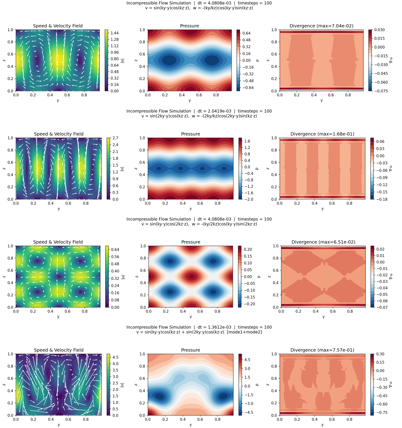
Figure 3.2: Resulting simulation results. Flow behavior for different parameterisations. Numerical calculations have been performed by using FFT and spectral decomposition.
